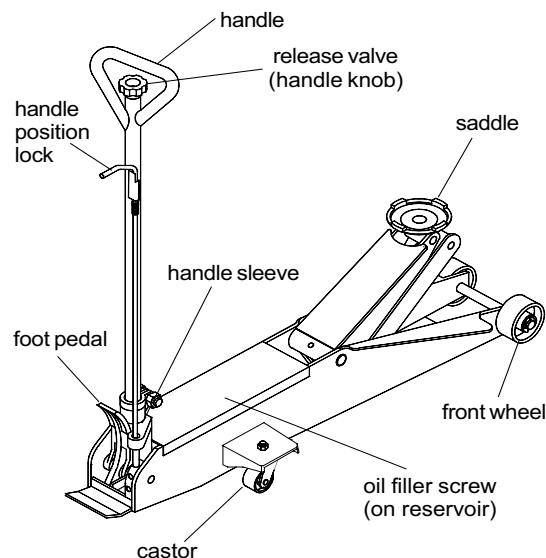
Figure 1 - Model 25057 & 25107 Components
