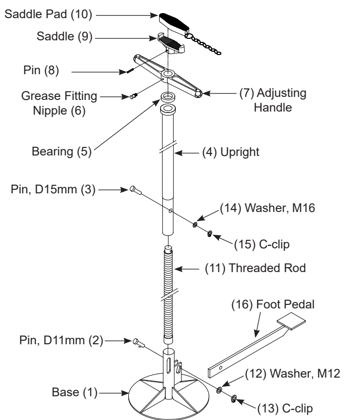
Figure 2 - BH5715 Nomenclature
