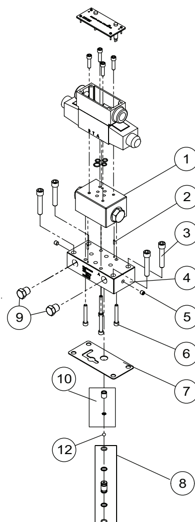
PS43L Parts Illustration
