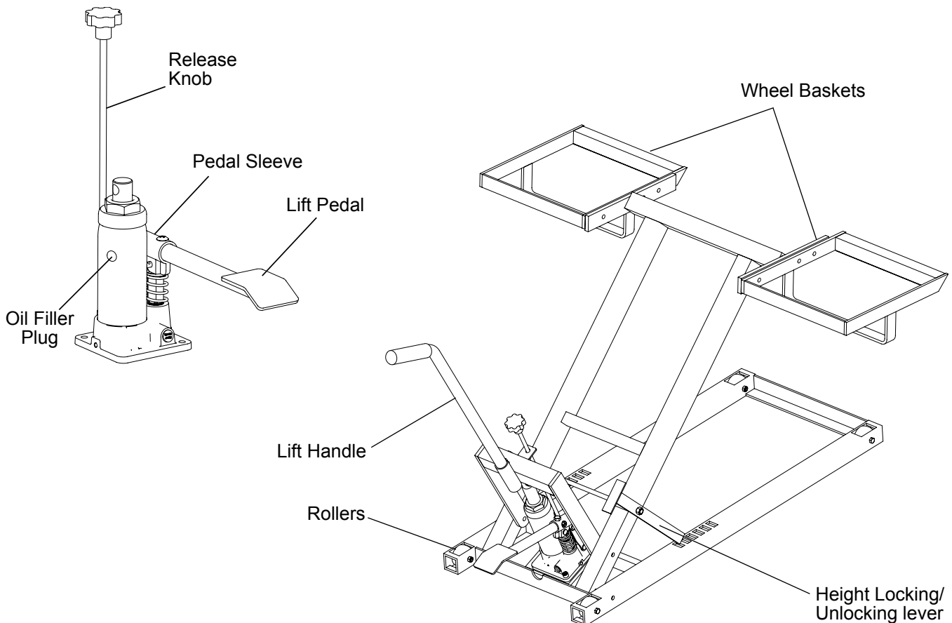
Mower Lift Nomenclature
