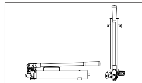
Figure 3 - Horizontal and Vertical Position
