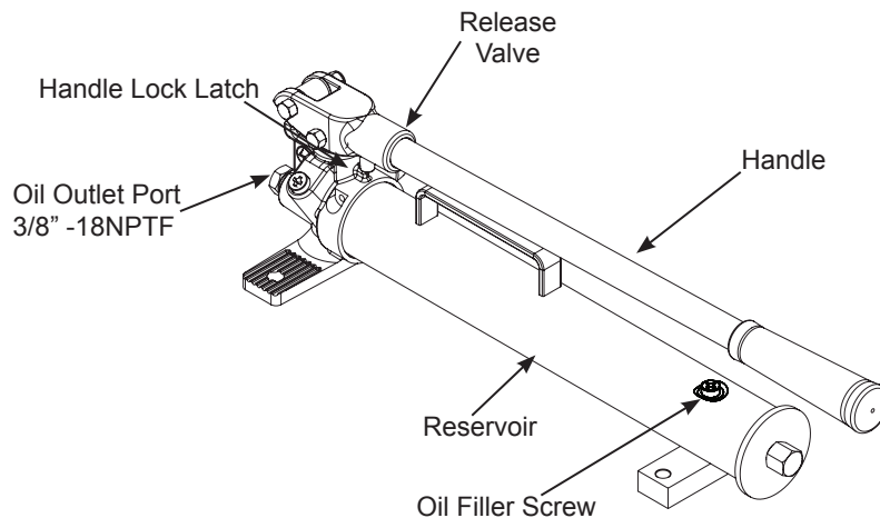
Figure 1 - Model ZP601S Components
