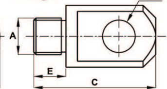
Plunger
